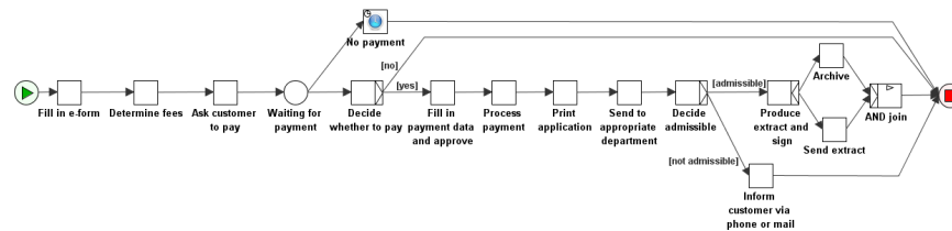
Fig. 1: GBA_1 YAWL model for Mun_E
