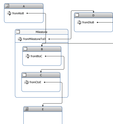
Figure 2. Graphical representation of the example of WCP18
